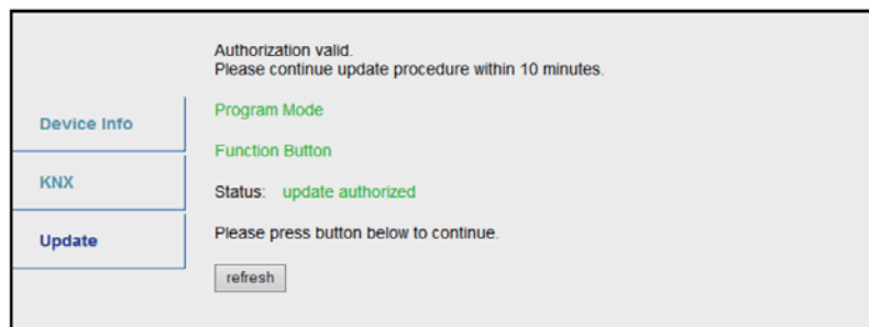
Figure 19: Update Authorized
