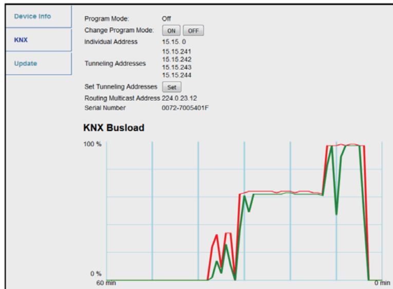
Figure 16: KNX Tab
